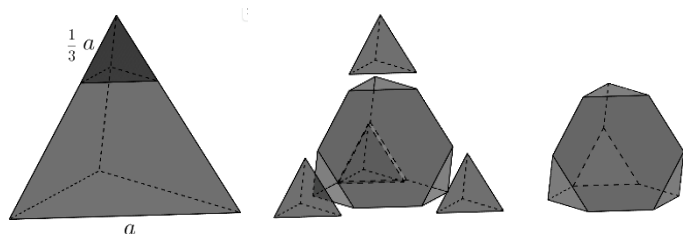
Tetraedro regular
